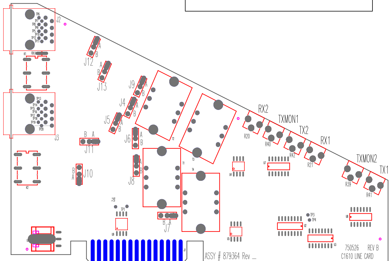
Figure 5 Line Card layout
