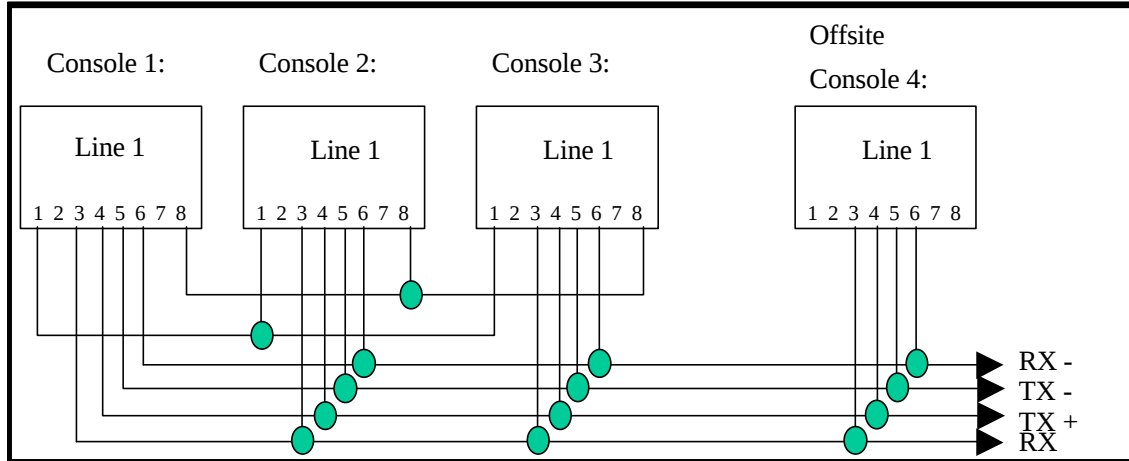
Figure 6 Crossmute Diagram
