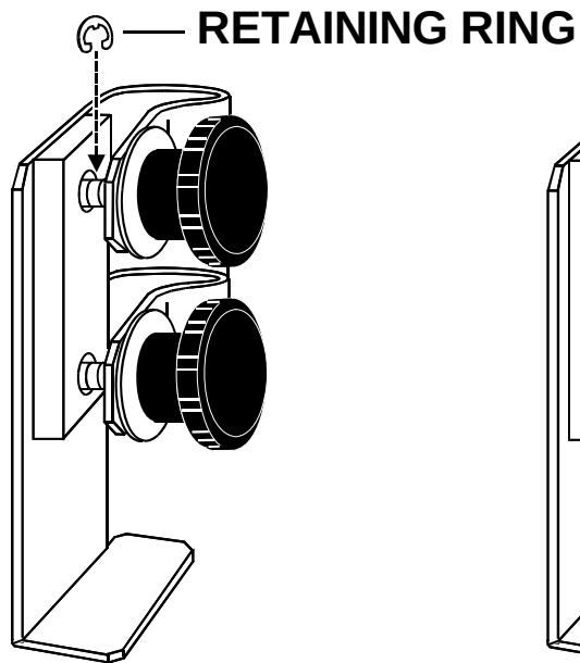
FINAL ASSEMBLY
