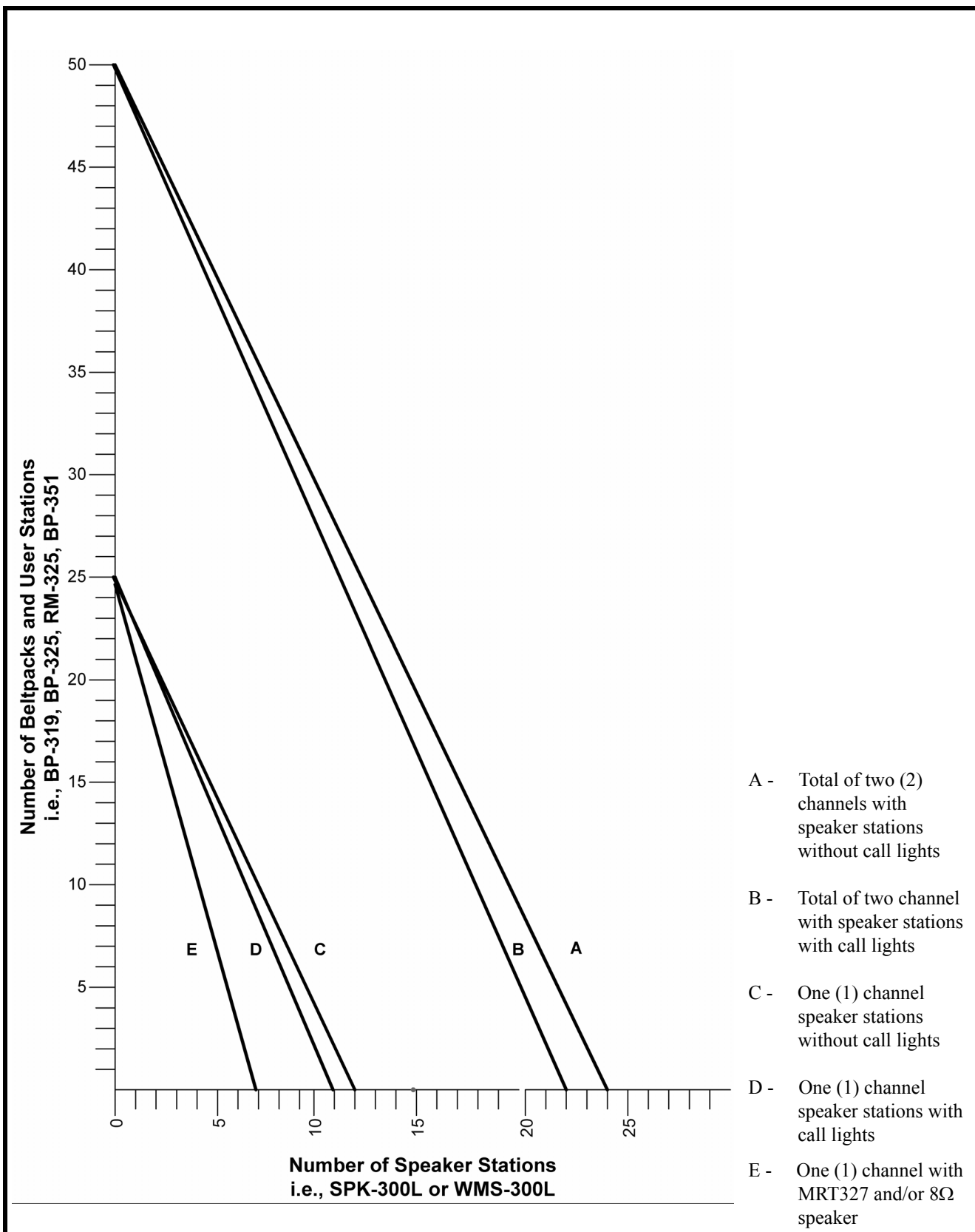
FIGURE 3. Capacity Graph
