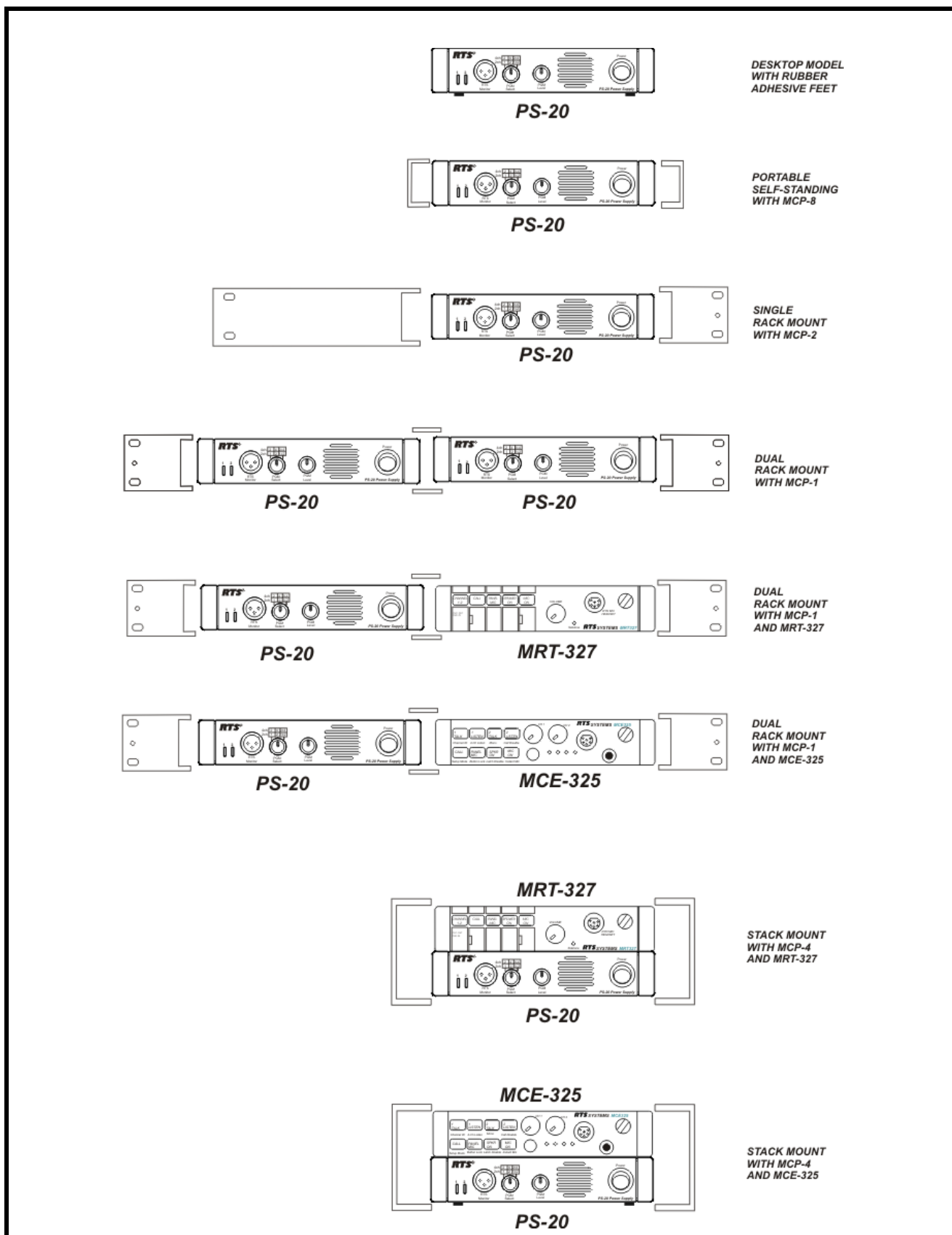
FIGURE 7. Rack Mount Configurations for the PS-20.
