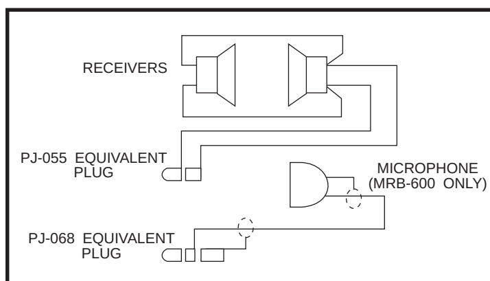
Schematic Diagram
