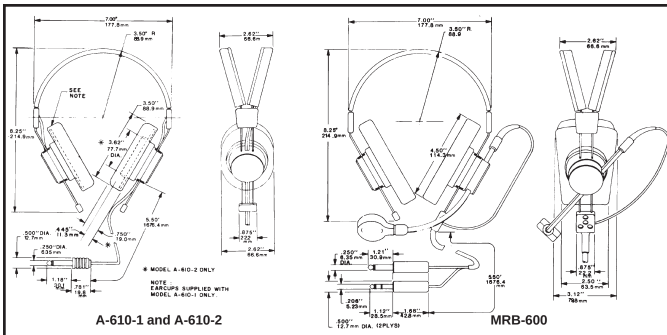
Dimension Drawings
