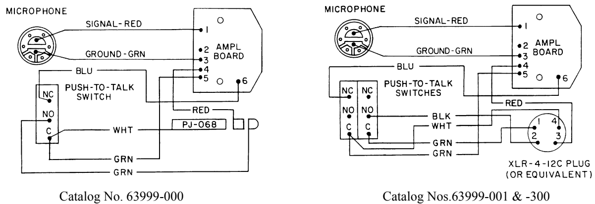
Figure 2: Wiring Diagrams
