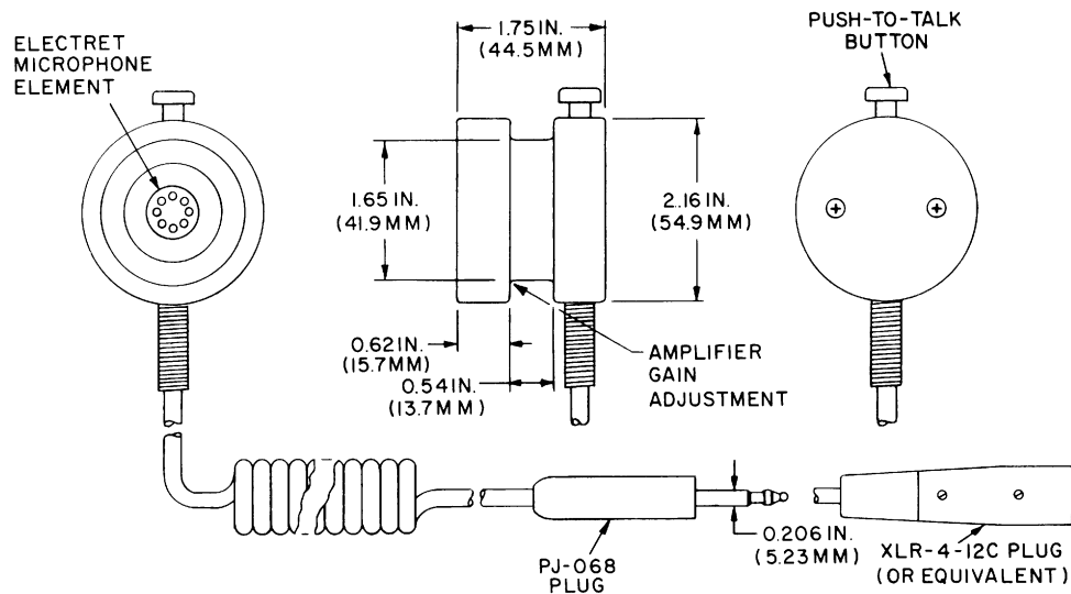
Figure 1: Dimensional Drawing
