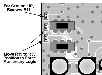
Figure 3: PC Board Detail
