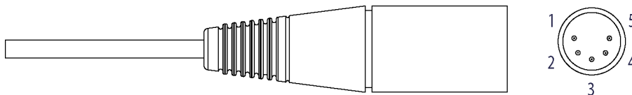
Figure 8.3: 5-pin XLR Connector
