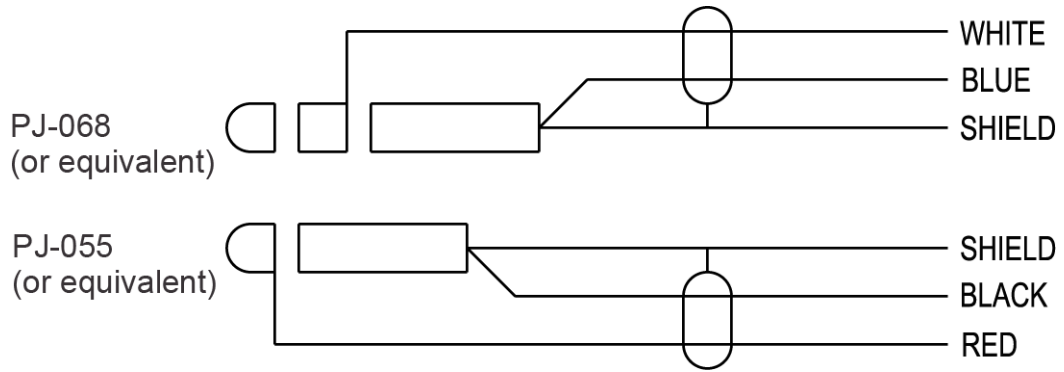
Figure 8.2: Wiring Diagram
